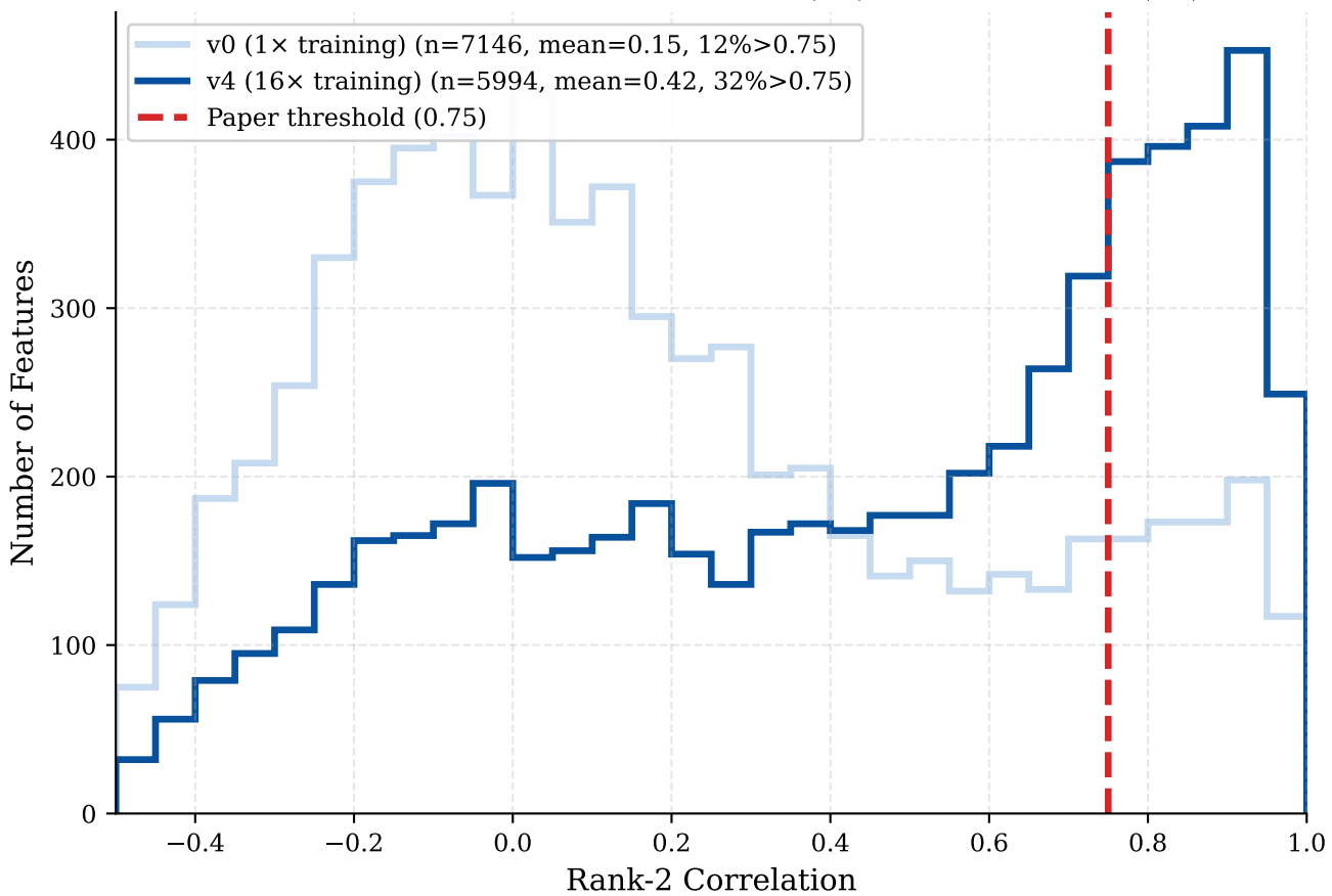
Rank-2 Correlation: Under-trained (v0) vs Well-trained (v4)
