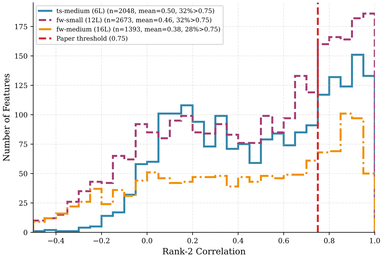
Rank-2 Correlation Distribution
