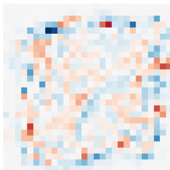
\lambda=-1.76
