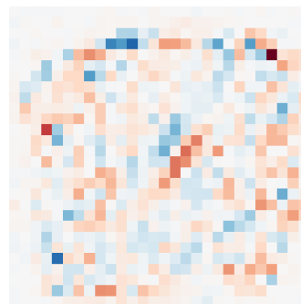
\lambda=-1.53
