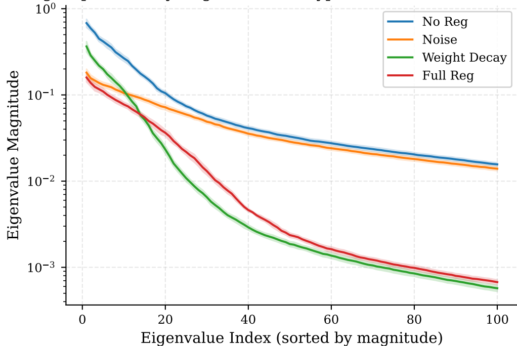
MNIST: Eigenspectrum by Regularization Type (shaded = 90% CI across classes)
