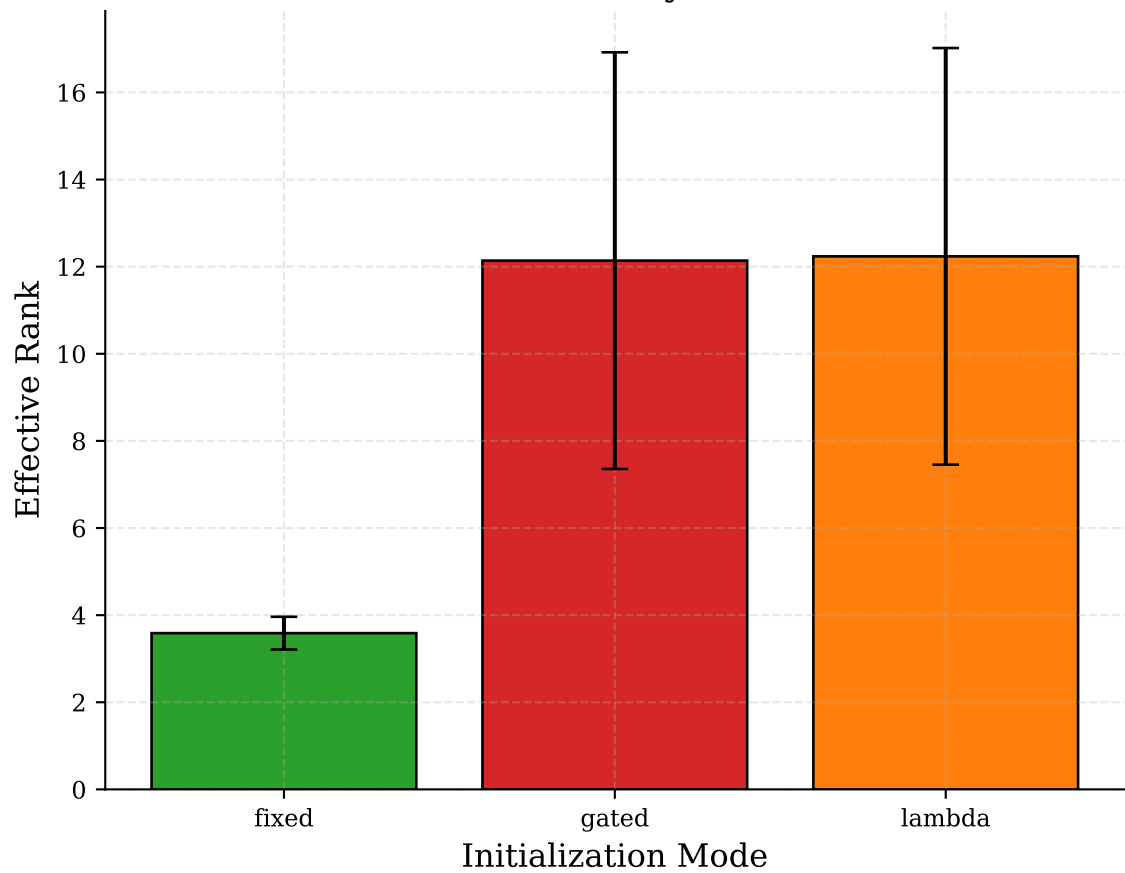
Effective Rank by Init Mode
