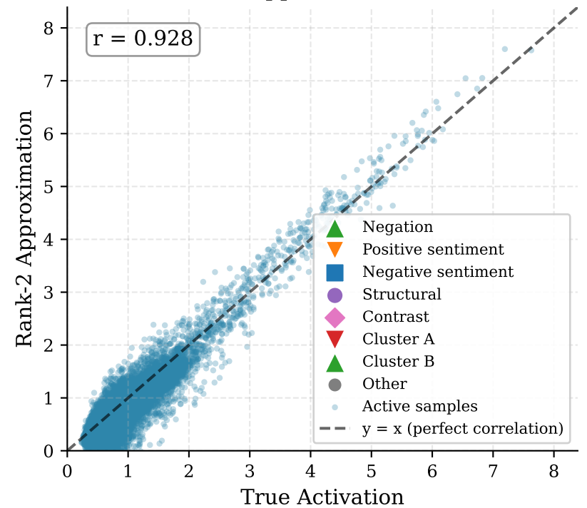
C) Activation vs Approximation (Feature 751)
