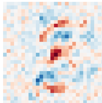
\lambda=-0.11
