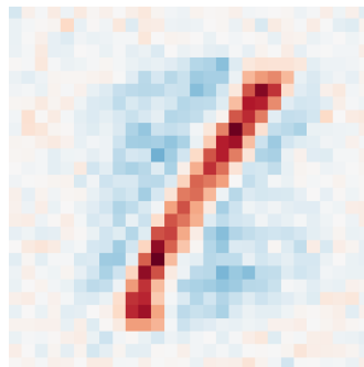
\lambda=0.10
