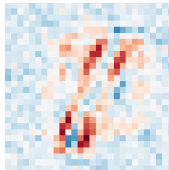
\lambda=0.07
