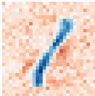
\lambda=-0.19
