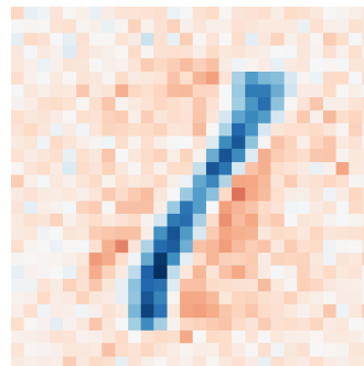
\lambda=-0.01
