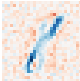
\lambda=0.17
