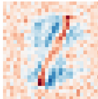
\lambda=0.14
