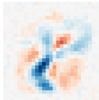
Class 8 (4.53)
