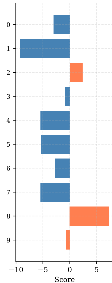
Class Scores
