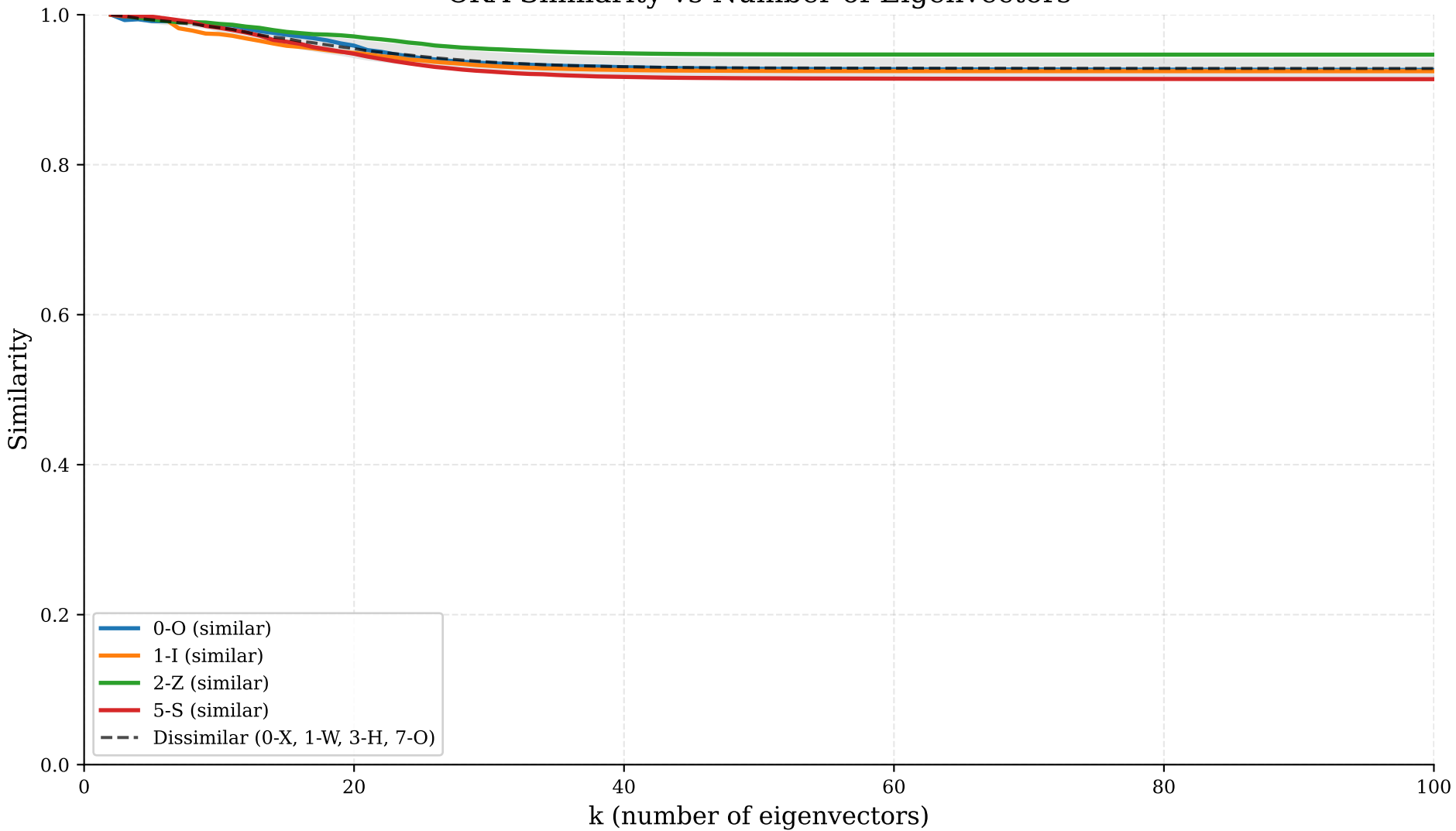
CKA Similarity vs Number of Eigenvectors
