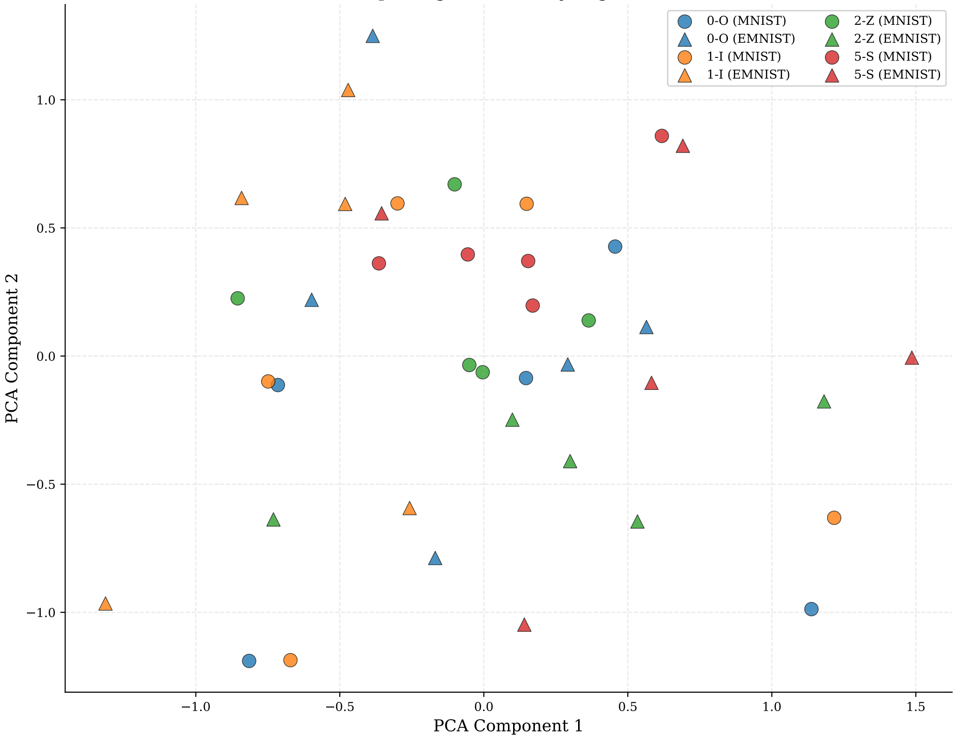
PCA of Top-5 Eigenvectors by Digit-Letter Pair
