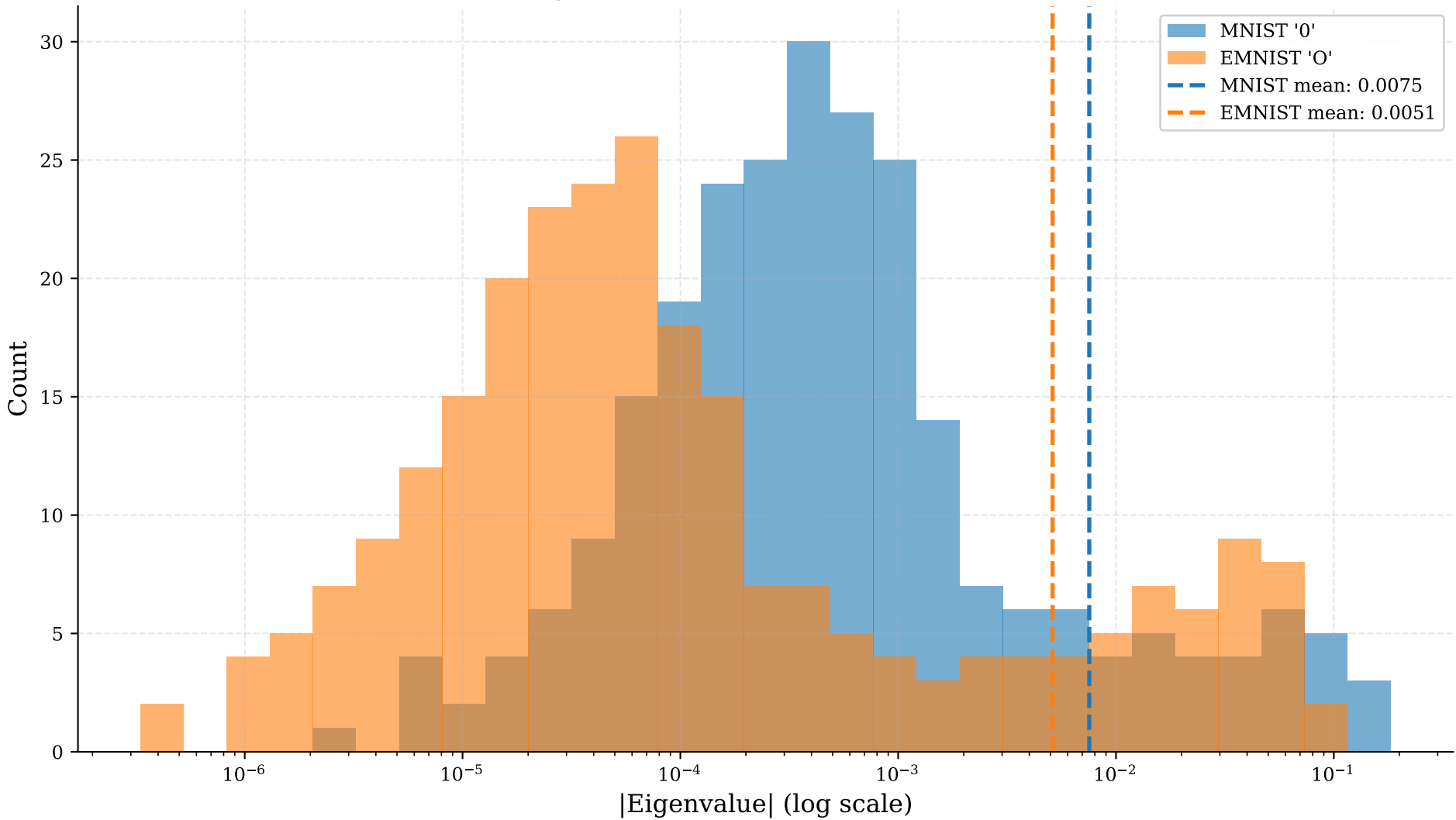
Eigenvalue Distribution: '0' vs 'O'
