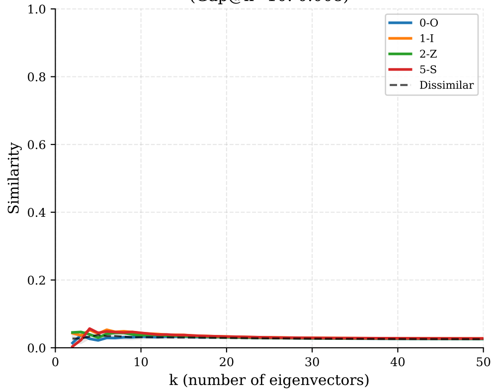
Eigenvalue-Weighted Cosine (Gap@k=10: 0.008)
