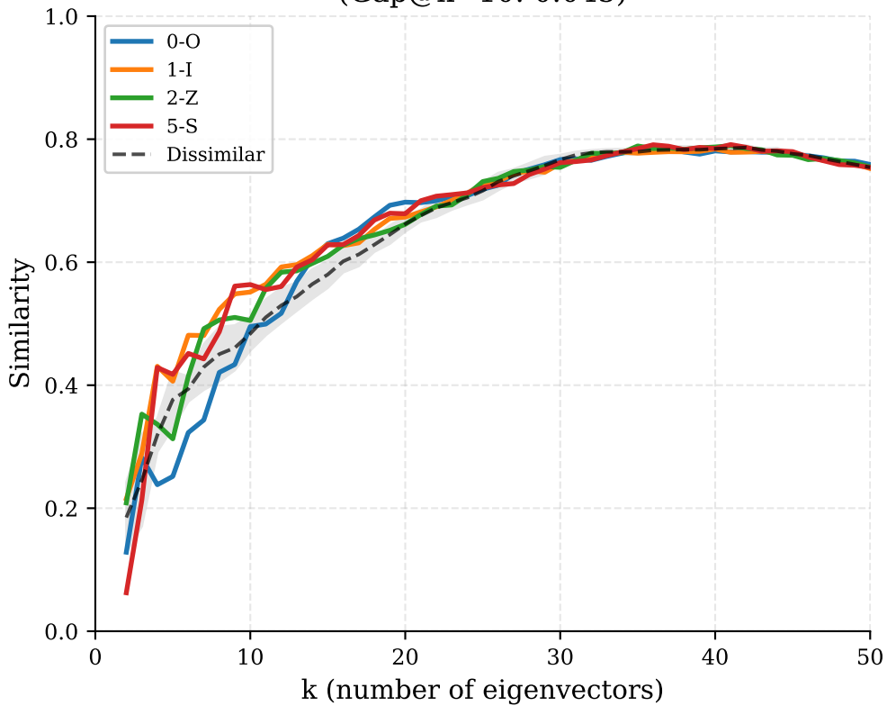
Mean Cosine (Principal Angles) (Gap@k=10: 0.045)
