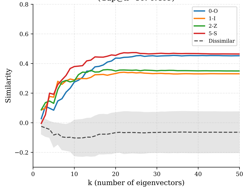
Quadratic Form (Gap@k=10: 0.409)
