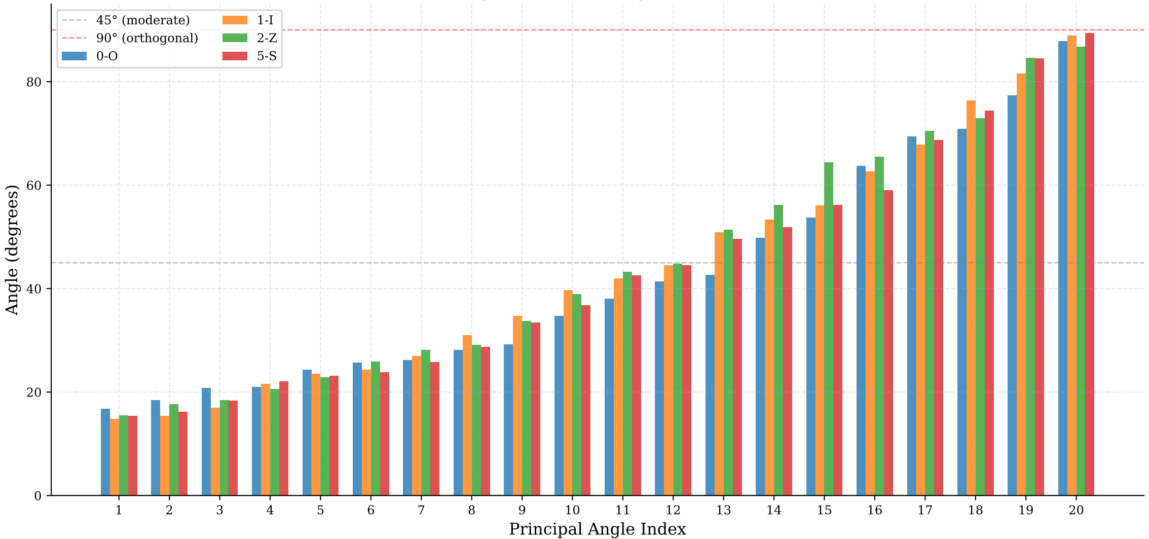
Principal Angles Between Digit-Letter Subspaces
