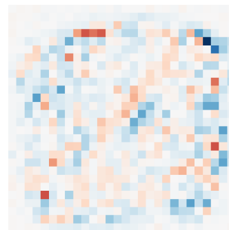
\lambda=-0.97
