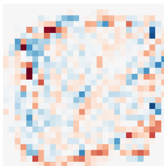
\lambda=-1.71
