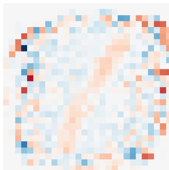
\lambda=0.94
