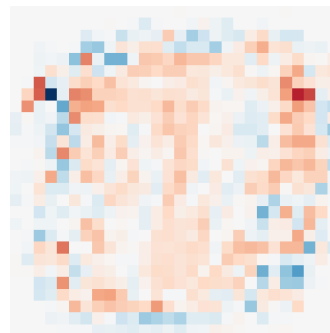
\lambda=0.45
