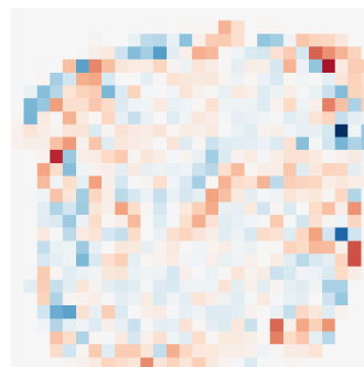
\lambda=-1.41
