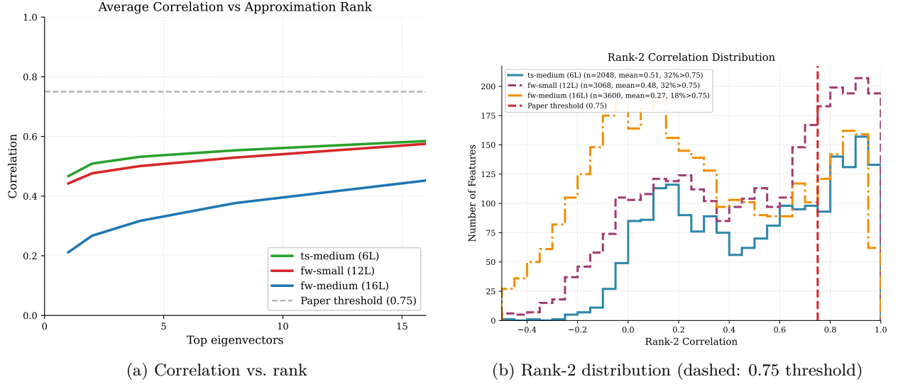
Figure 3: Low-rank correlation analysis (Paper Figure 9). Configurations: ts-medium (layer 4, \text{exp}=4 , n=2,048 ), fw-small (layer 8, \text{exp}=4 , n=3,068 ), fw-medium (layer 7, \text{exp}=8 , n=3,600 ). Only features with \geq 50 activations included. Mean rank-2 correlations range 0.27–0.51; only 18–32% exceed the 0.75 threshold vs. paper’s 69%.
