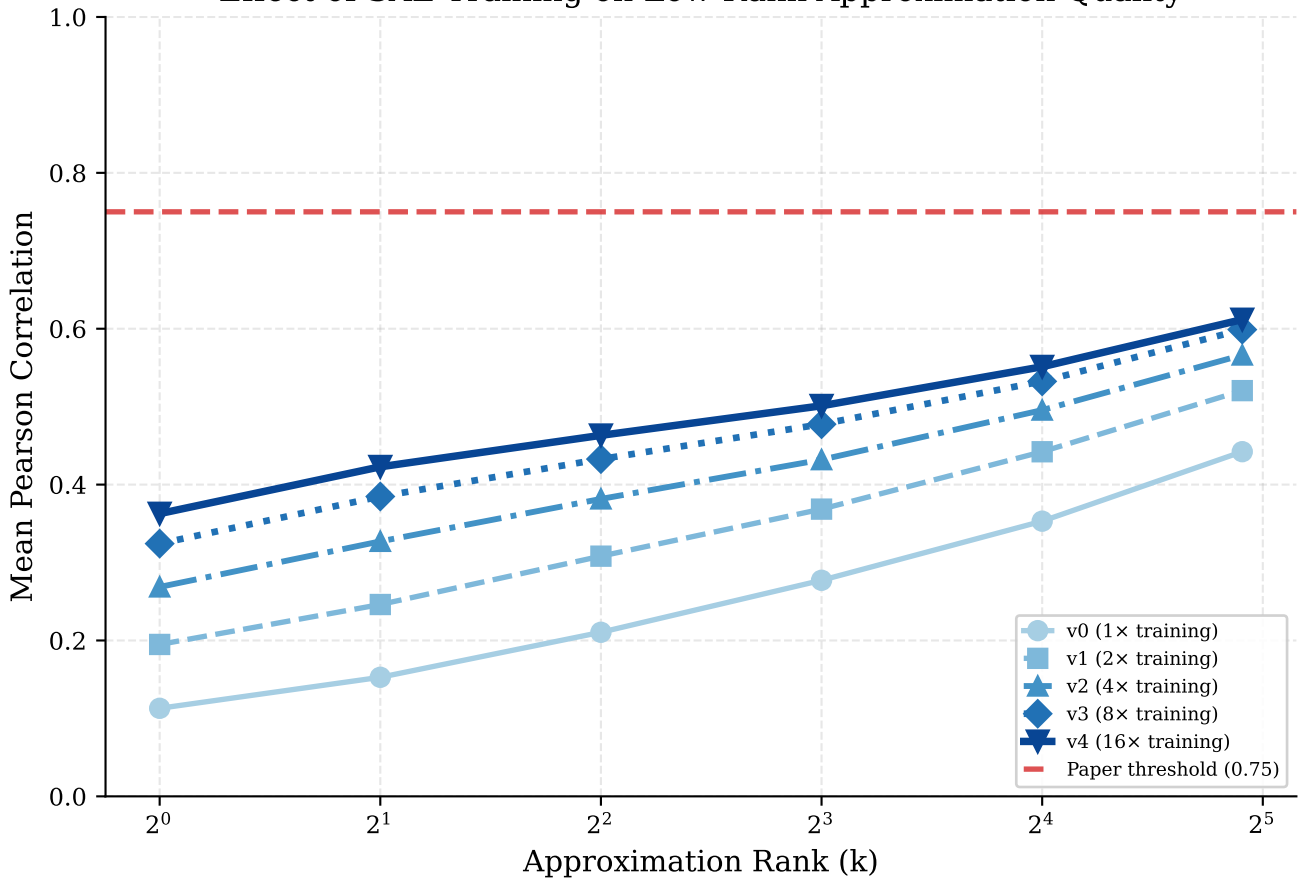
Effect of SAE Training on Low-Rank Approximation Quality
