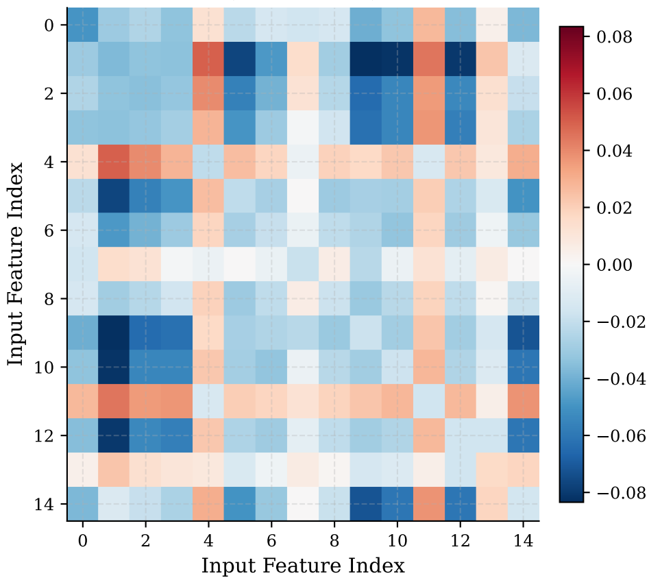
Interaction Submatrix (Feature 751)
