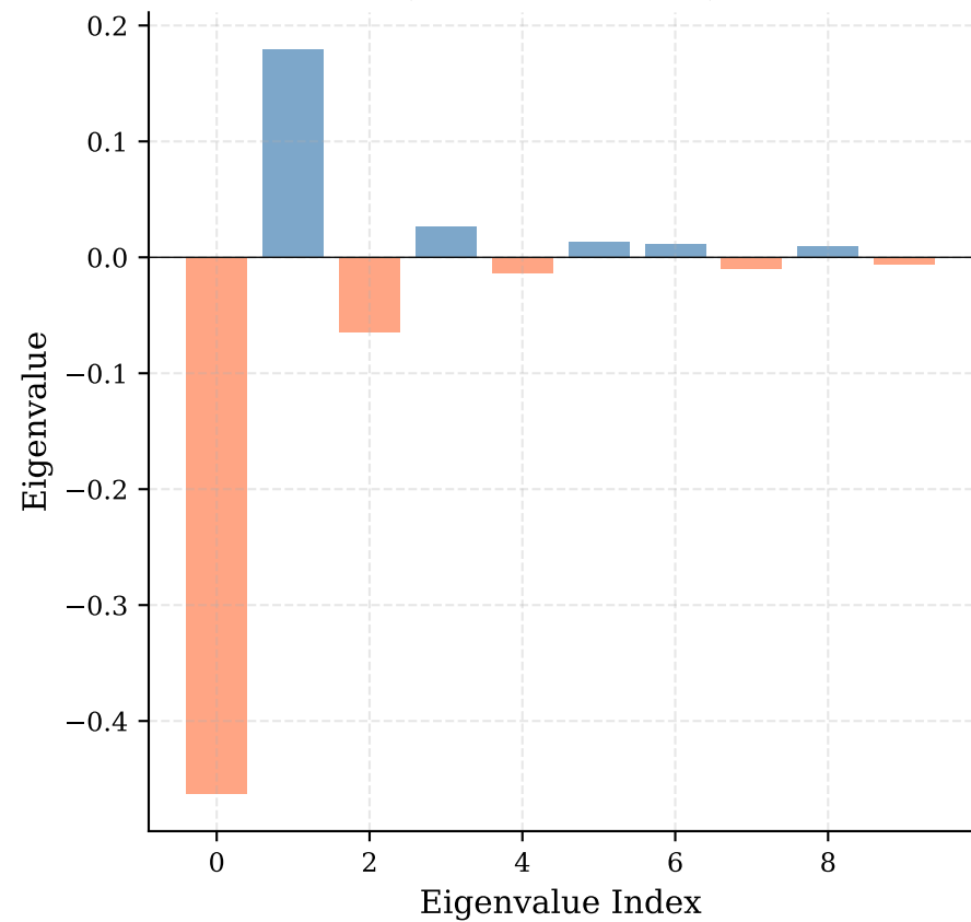
Eigenvalue Spectrum (AND-score: 0.96)
