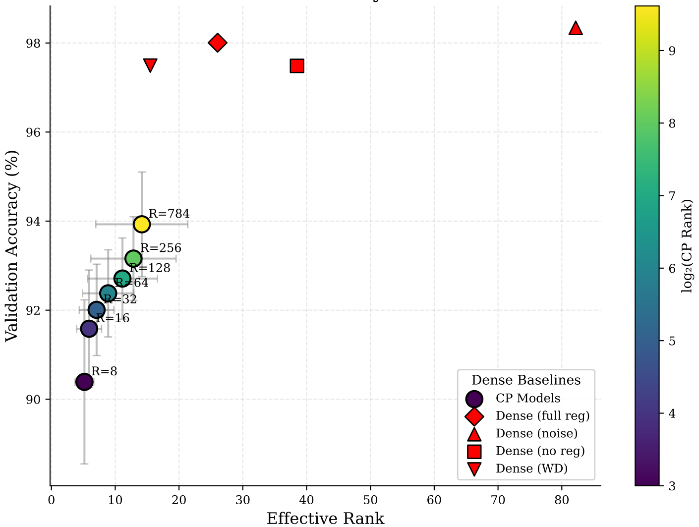
CP Rank vs Accuracy Trade-off
