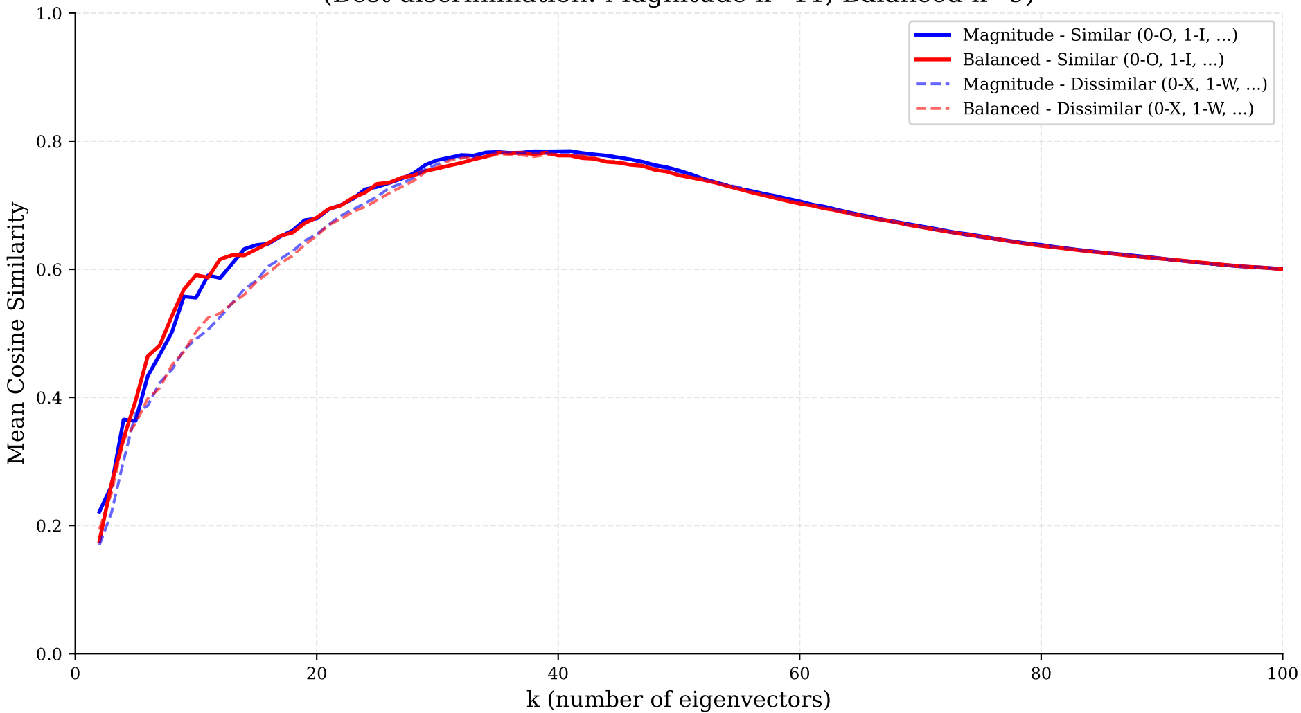
Selection Method Comparison (Best discrimination: Magnitude k=11, Balanced k=9)
