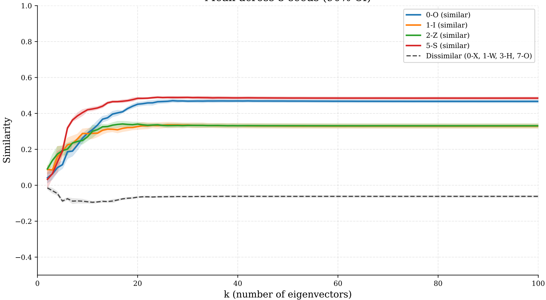
Quadratic Form Similarity vs Number of Eigenvectors Mean across 5 seeds (90% CI)
