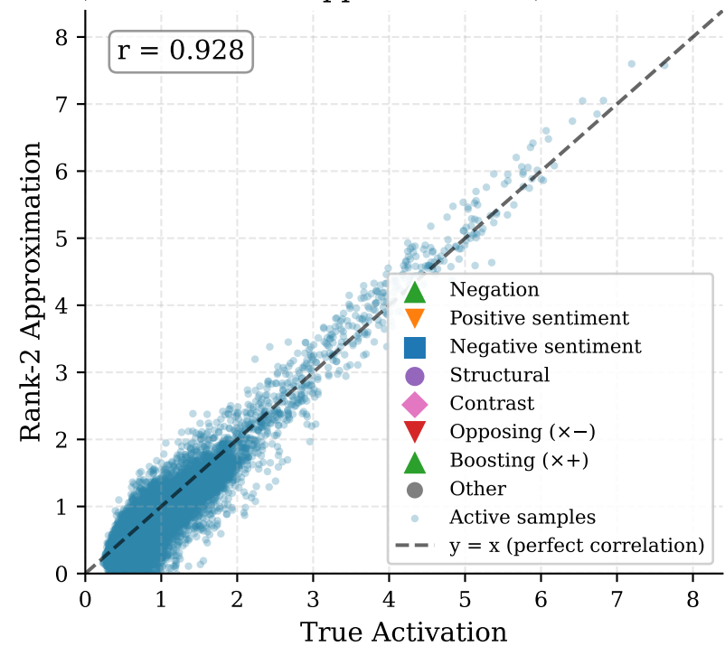
C) Activation vs Approximation (Feature 3834)
