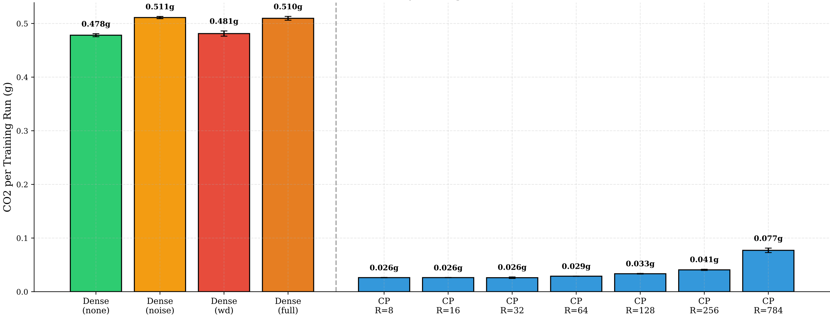
Environmental Cost: Dense vs CP by Configuration (mean \pm std across seeds)
