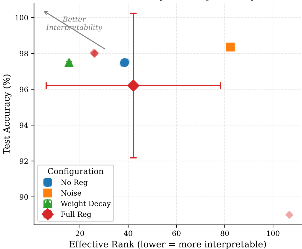
MNIST: Accuracy vs Interpretability
