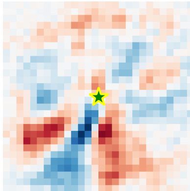
EMNIST Eigenvec #2 \lambda = -0.145 CoM=(13.5, 13.5)
