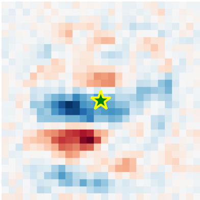
MNIST Eigenvec #1 \lambda = -0.300 CoM=(13.5, 13.5)
