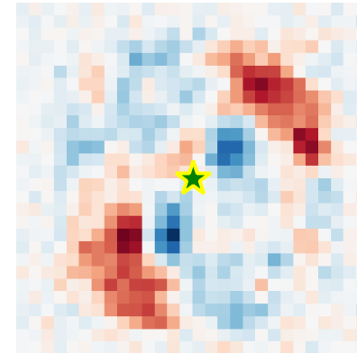
MNIST Eigenvec #3 \lambda = -0.204 CoM=(13.6, 13.6)
