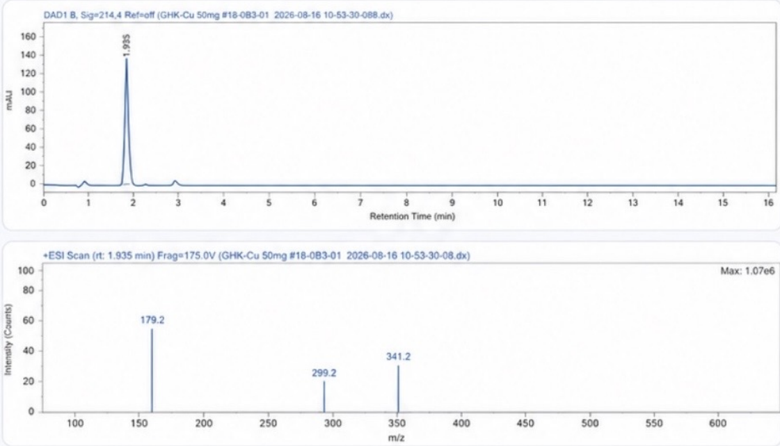
HPLC Chromatogram · Retention Time 1.935 min
