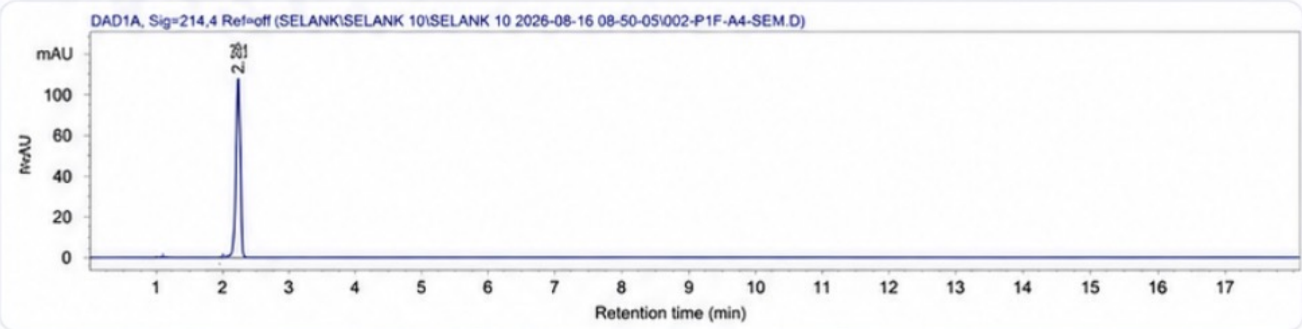
HPLC Chromatogram • Retention Time 2.291 min
