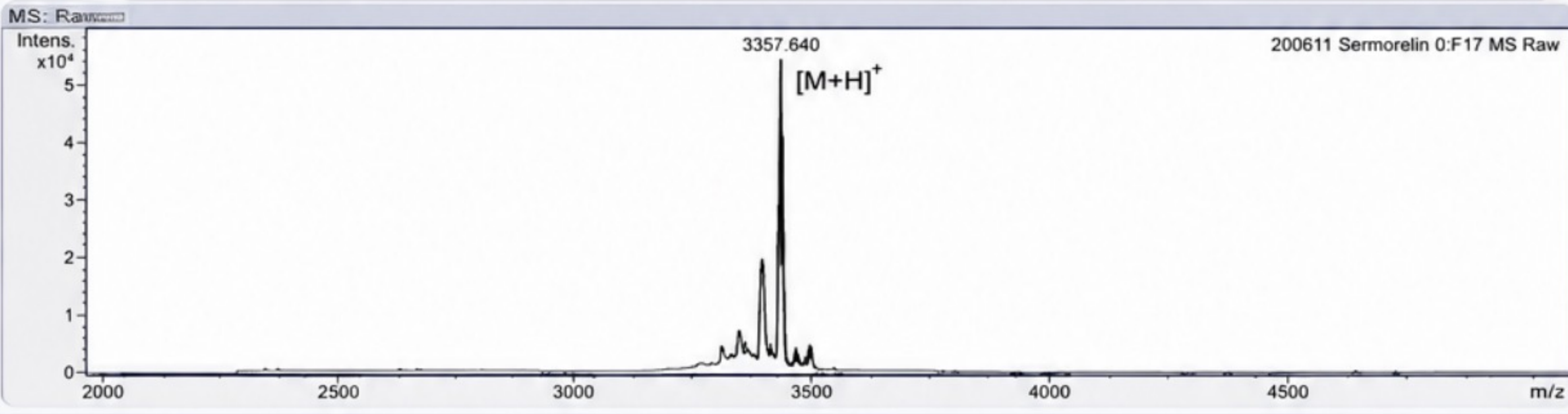
Mass Spectrum (MALDI-MS)
