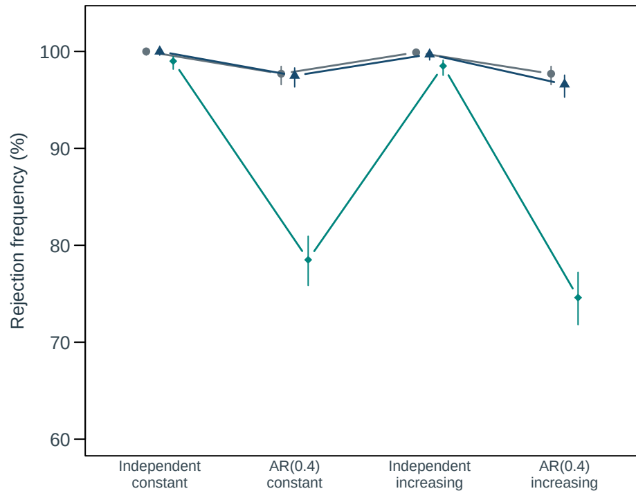
Power (change 0.14 degrees C/decade)
