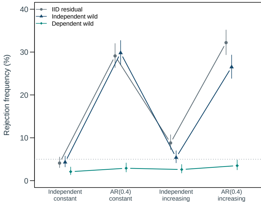
Null rejection (nominal 5%)
