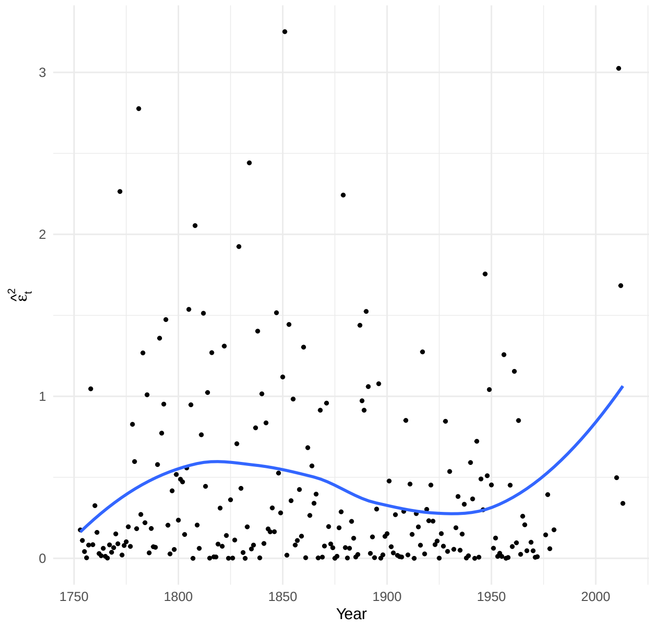
Squared Residuals over Time
