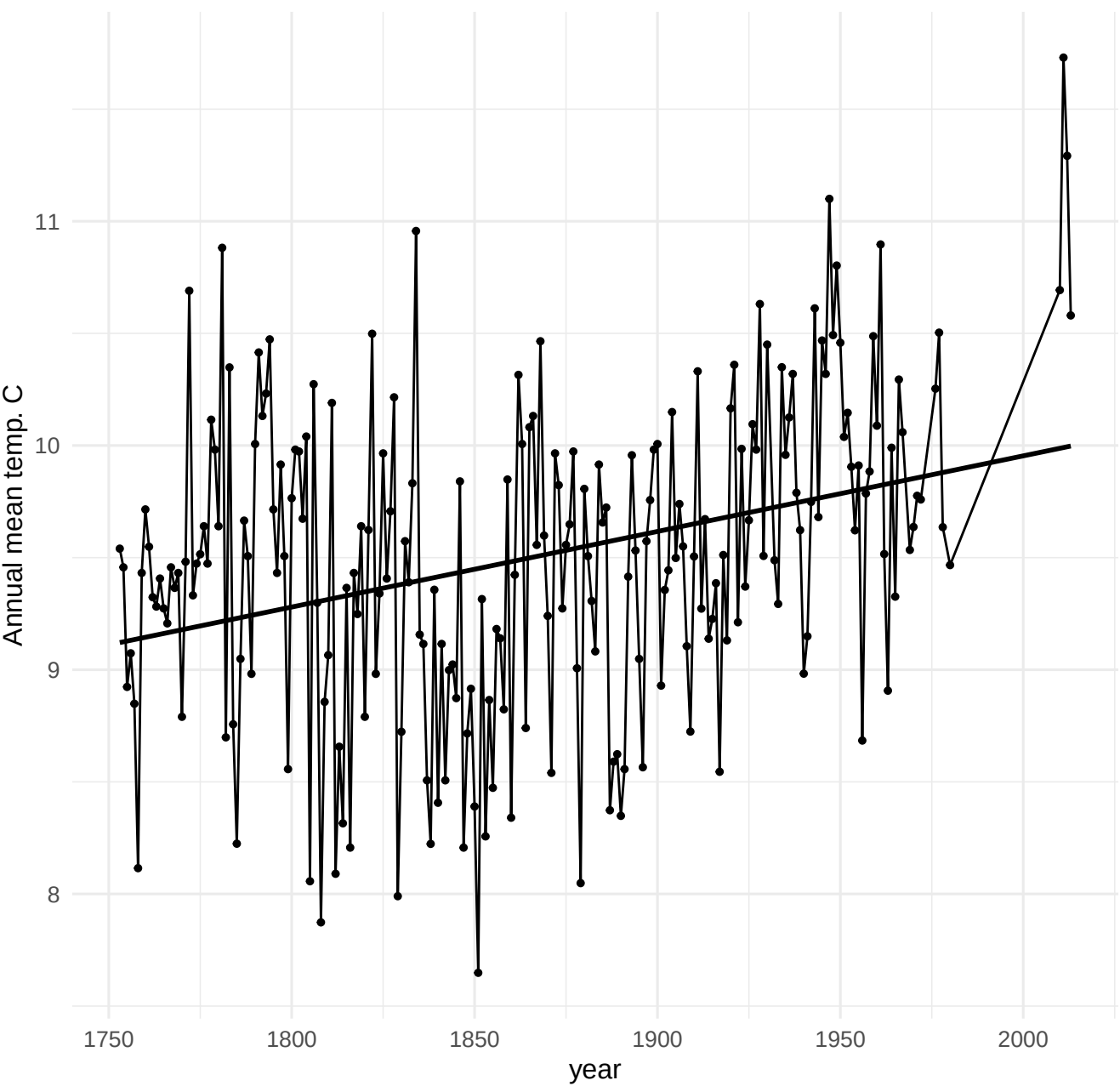
Geneva temp. series with linear trend
