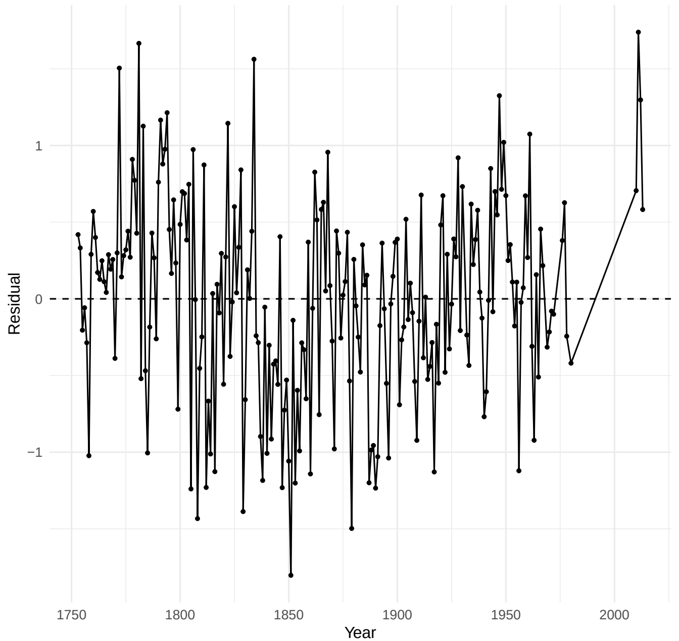
Residuals from Linear Trend Model
