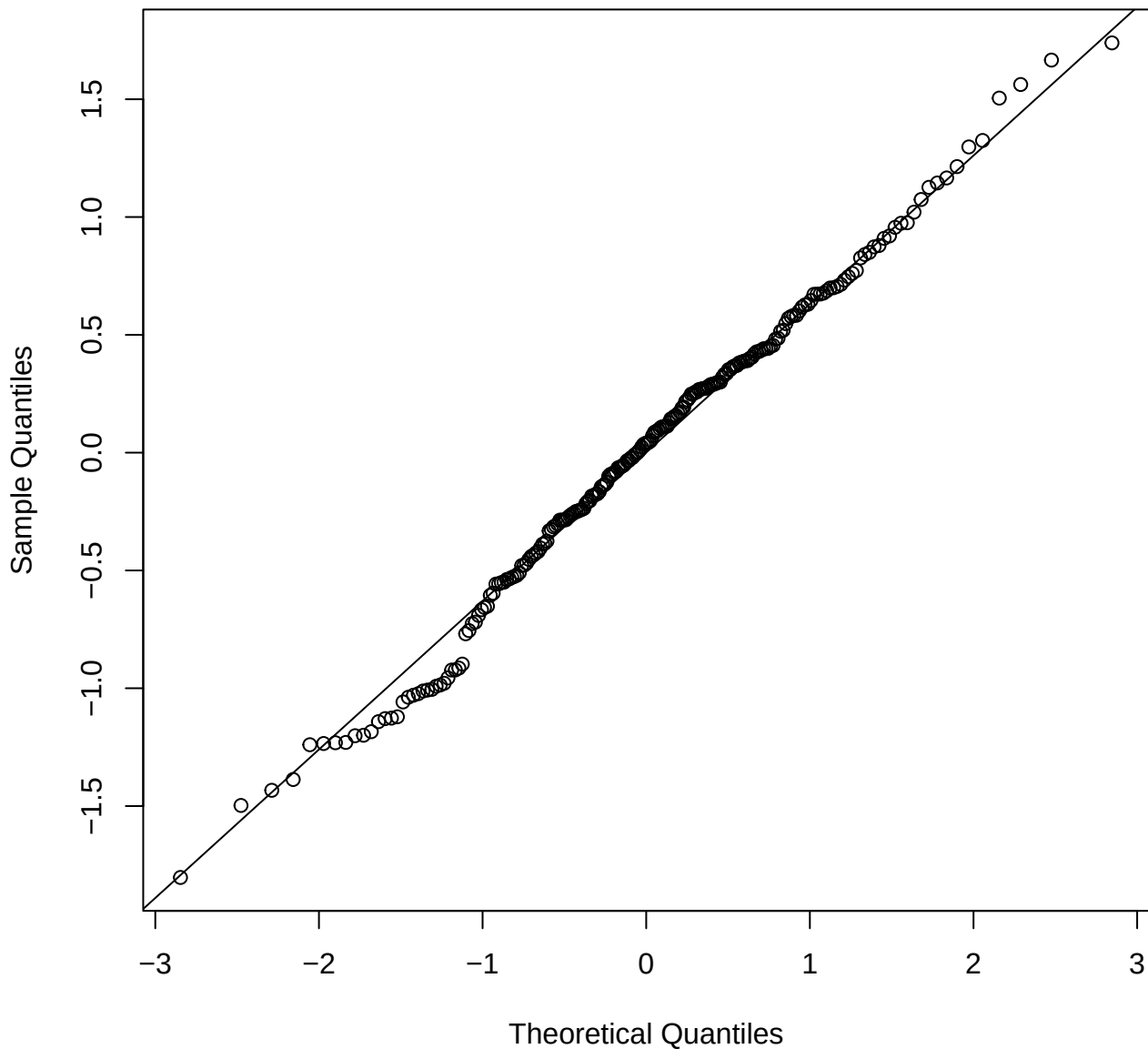
Normal QQ Plot of Residuals
