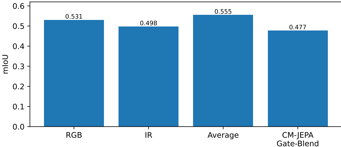
U-Net/MobileNetV2 semantic segmentation results on MSRS
