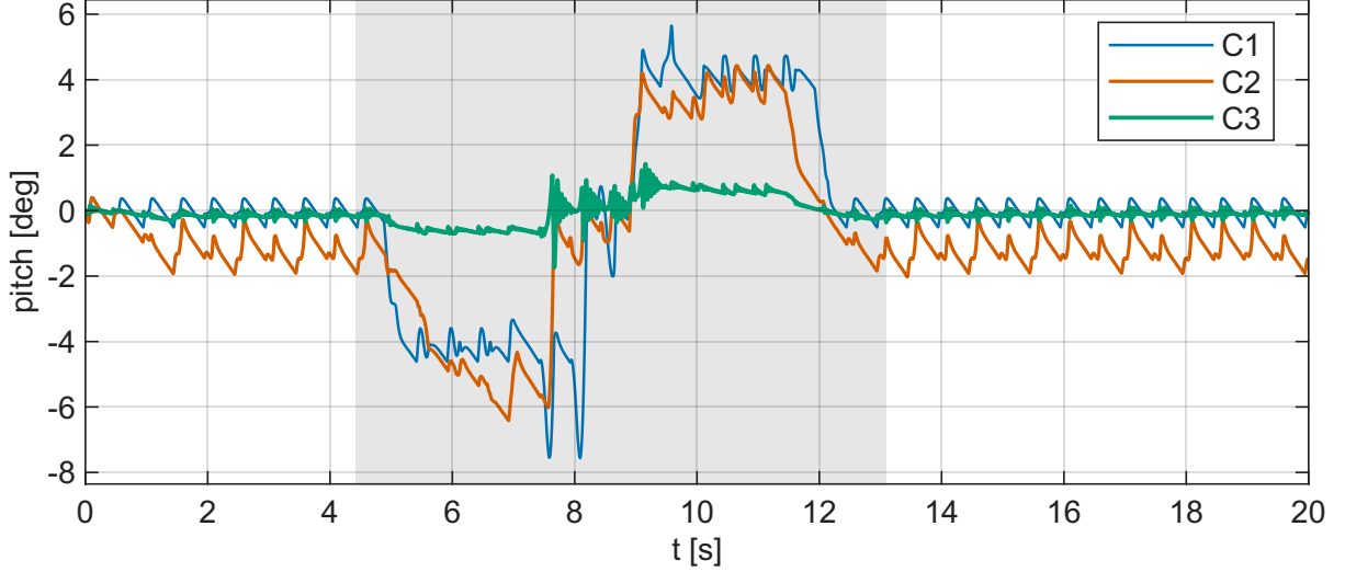
Figure 4: Body pitch while crossing the single obstacle (T5). In grey the window in which at least one foot is on the obstacle, identified kinematically. Outside that window the three curves oscillate around zero with the step amplitude; inside, C1 and C2 make an excursion of several degrees in both directions — first nose up while the front legs climb onto the step, then nose down when the rear ones climb onto it — while C3 stays within about one degree throughout the crossing. It is the same difference that Table 8 reports as -73\% peak pitch.
