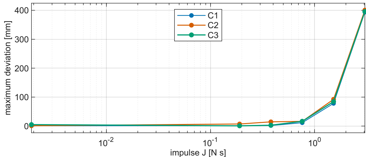
Figure 6: Maximum lateral deviation versus the amplitude of the applied impulse (T7), with a logarithmic abscissa to cover the three decades of the sweep. The three curves are practically indistinguishable over the whole range: up to about 0.7\text{ N s} the deviation stays at a few millimetres for all, beyond that it rises sharply to almost 400\text{ mm} without any of the three controllers standing out from the others. It is the direct representation of a common architectural gap: neither terrain search nor the attitude loop acts on this disturbance.
