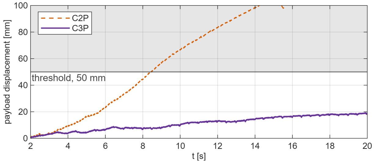
Figure 8: Displacement of the package from the reference on the 8° ramp (T4), with the attitude loop off (C2P) and on (C3P). The line and the grey band mark the 50 mm clearance between cube and tray: above it, the cube is no longer contained by the tray. C2P exceeds it after 8.4 s and continues without coming back — beyond the frame the curve reaches tens of metres, because the cube leaves the robot and falls. C3P stays below 20 mm for the whole run. The measurement starts at 2 s, after the settling transient on which the reference is defined.
