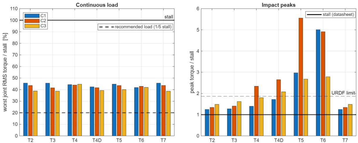
Figure 7: Torque demanded at the joints versus the AX-12A limits, per task and controller. Two distinct regimes must be read: the RMS torque of the most loaded joint, which describes walking and stays steadily below stall but above the continuous load recommended by the manufacturer, and the peak torque, which exceeds stall at stance impacts. The corresponding numerical values are in Table 12.
