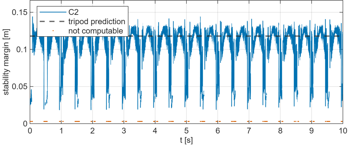
Figure 10: Stability margin of controller C2 in straight walking on flat ground (T2) at nominal speed (0.12 m/s, period 1 s), for ten cycles. The margin is the signed distance of the ZMP from the nearest side of the polygon formed by the stance feet: positive if the ZMP is inside the polygon.
