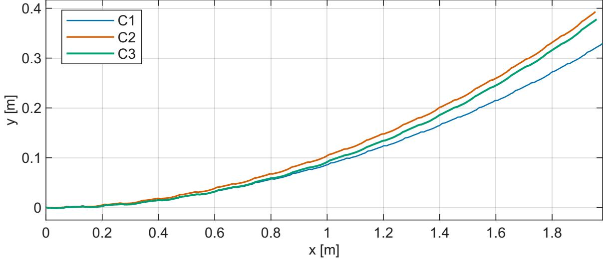
Figure 3: Trajectory of the centre of mass in the horizontal plane with a yaw command of +0.1 rad/s (T3). The three curves overlap almost everywhere: the yaw command is followed in the same way by the three controllers, and the differences in Table 7 on this task concern body attitude, not the path. The two axes have different scales — almost two metres on the abscissa versus four decimetres on the ordinate — so the lateral deviation appears much more pronounced than it is.
