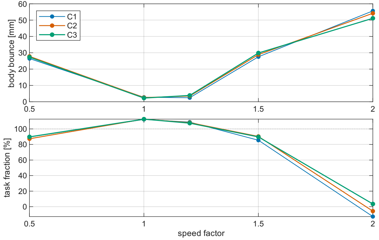
Figure 2: Speed sweep (T2) for the three controllers: vertical body bounce (top) and fraction of the task covered (bottom) versus the commanded speed factor.
