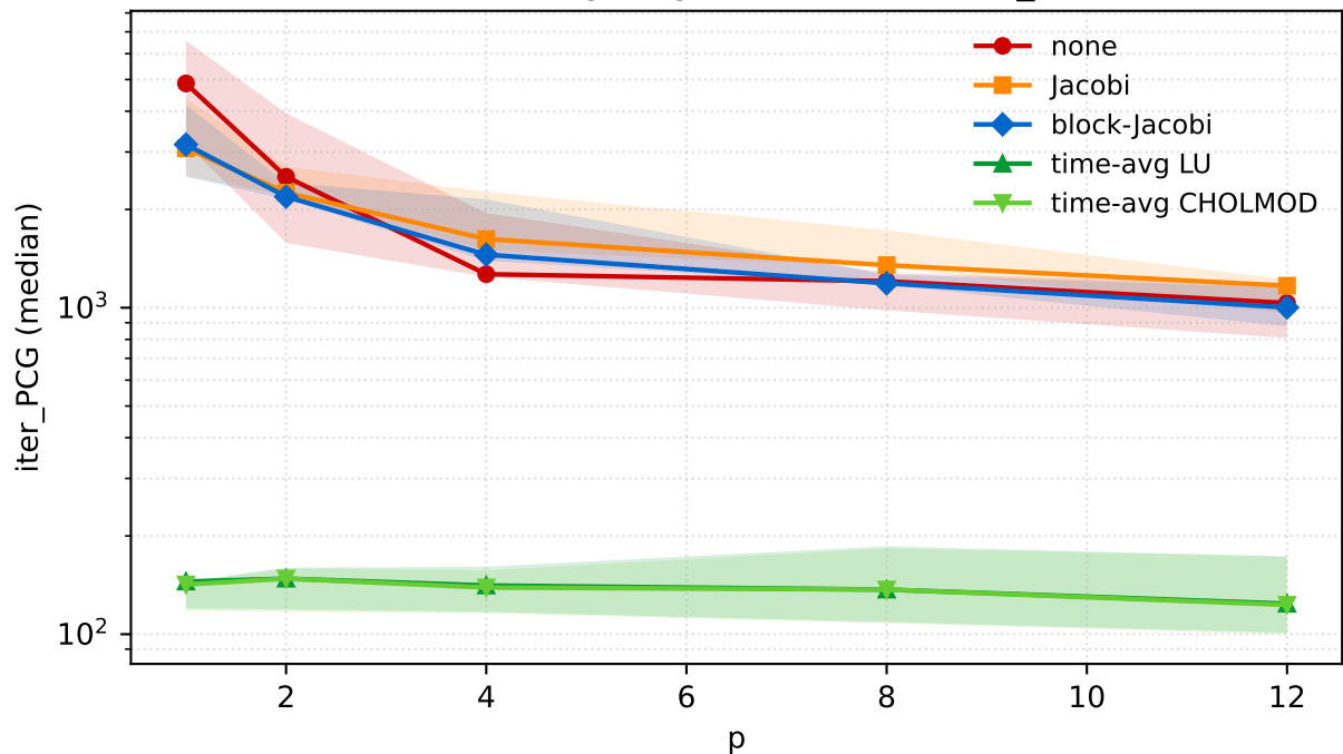
PCG iterations vs VAR lag length ( n=5 , T=480 , \sigma_{SV}=0.3 , \lambda=1e4 )
