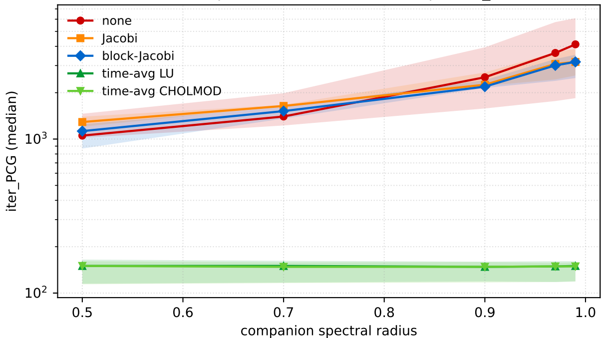
PCG iterations vs VAR persistence ( n=5 , T=480 , p=2 , \sigma_{SV}=0.3 , \lambda=1e4 )
