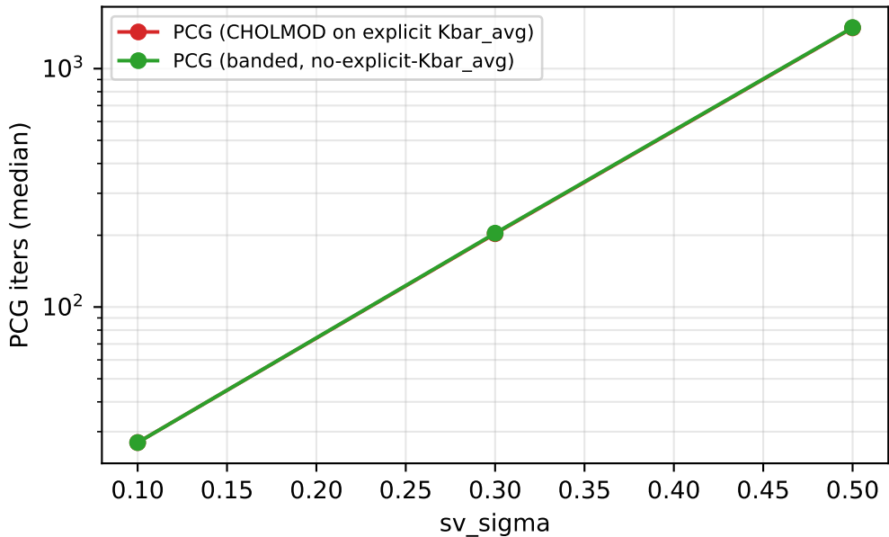
PCG iteration alignment ( n=5 , T=1920 , p=2 , \text{lam}=1\text{e}4 )
