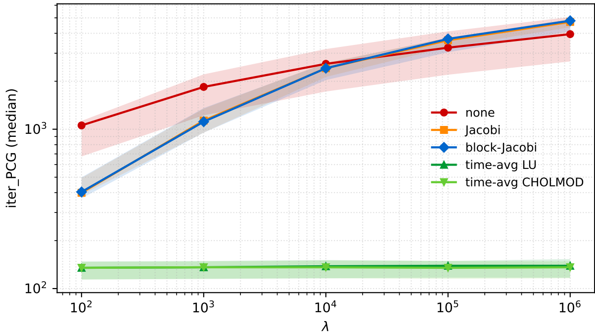
PCG iterations vs \lambda ( n=5 , T=480 , p=2 , \sigma_{SV}=0.3 )
