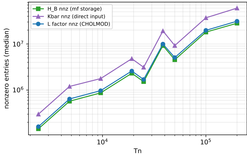
Storage breakdown
