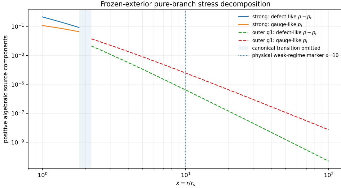
Figure 15: Positive algebraic defect-like and gauge-like source components on the frozen pure branches. The transition is omitted because it leaves this positive cone; x = 10 marks a regime label, not a formula switch.
