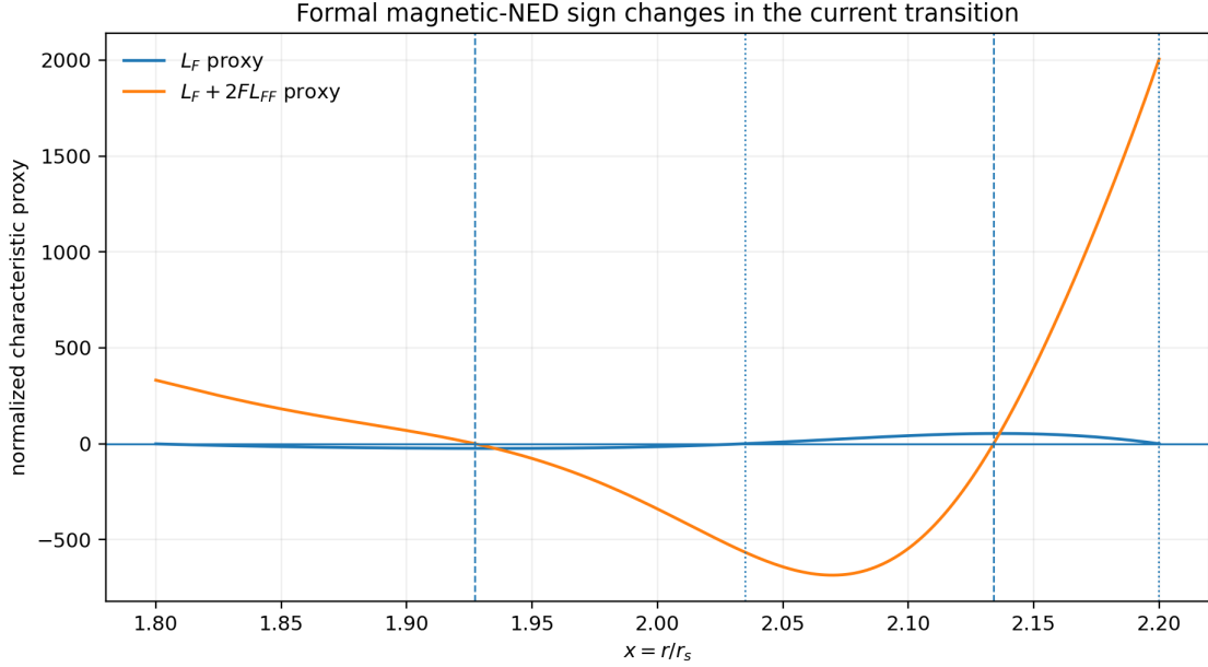
Figure 14: Formal magnetic-NED kinetic/characteristic proxies across the canonical transition, using the corrected sign convention.
