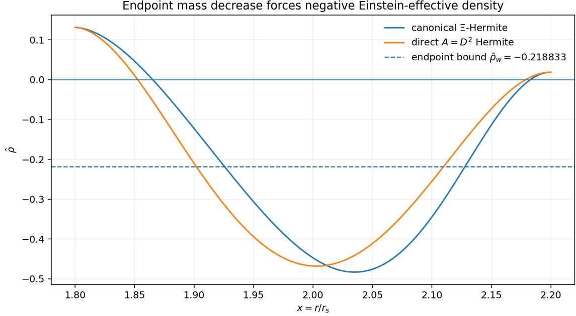
Figure 11: Changing the interpolated variable changes the transition shape but not the endpoint mass no-go. The dashed line is the interpolation-independent weighted-mean bound.
