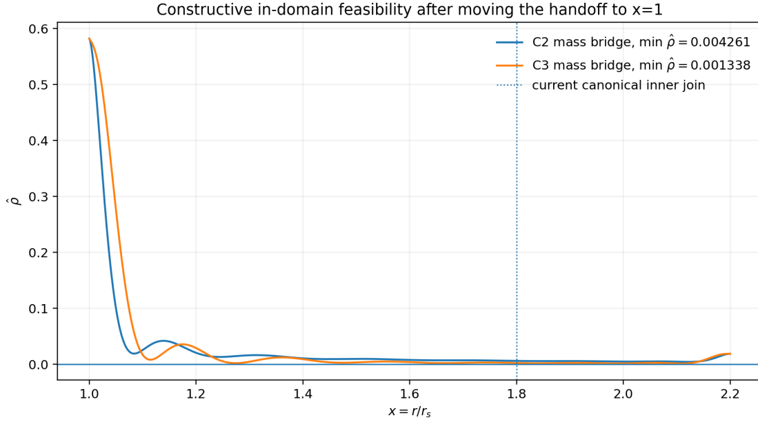
Figure 13: Two in-domain positive-density constructions and off-domain stronger-energy-condition feasibility witnesses. The fixed- x_1 NEC theorem prevents interpreting these as a full ordinary-matter rescue.
