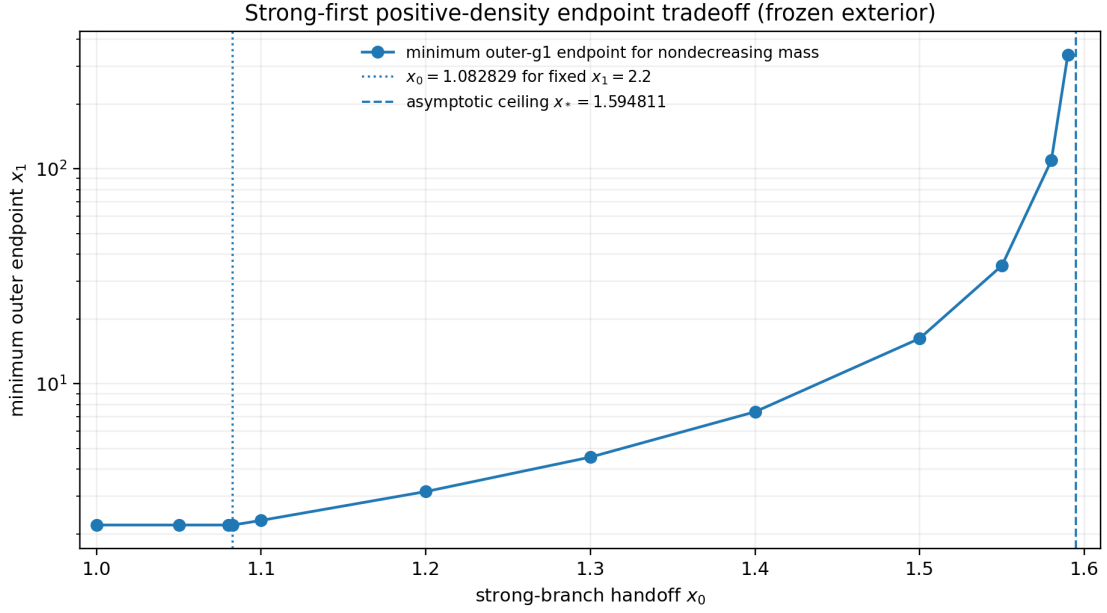
Figure 12: Strong-first endpoint tradeoff for nondecreasing Einstein mass. The required outer endpoint grows rapidly and diverges as x_0 \rightarrow x_*^- .
