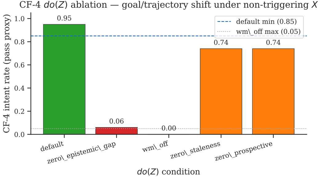
Figure 2: CF-4 ablation: strongest D1 ATT-E proxy. Proof-protocol acceptance yields e_endo_support=partial at best.
