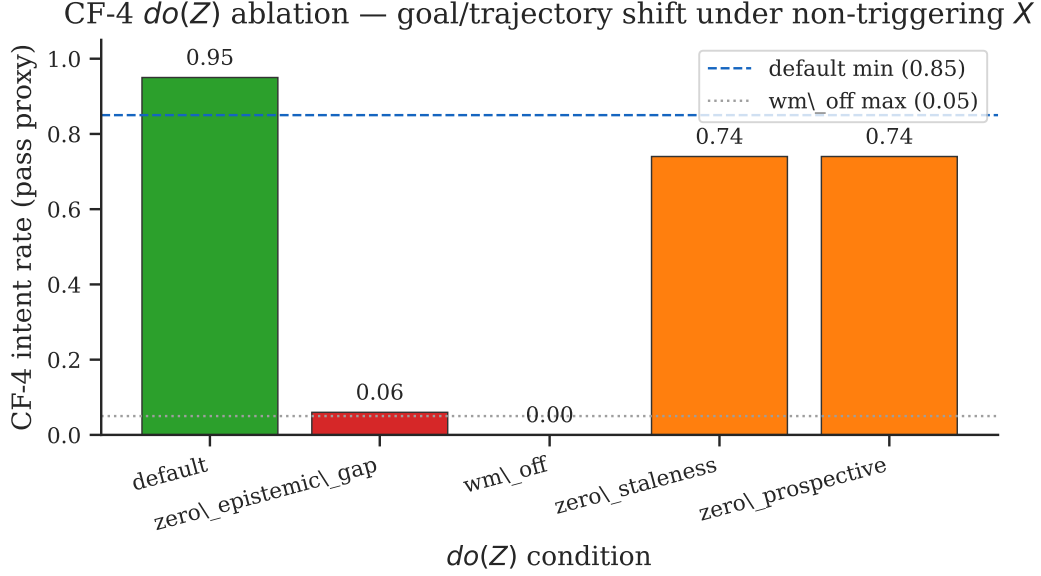
Figure 1: CF-4 ablation: strongest D1 ATT-E proxy. Proof-protocol acceptance yields e_endo_support=partial at best.
