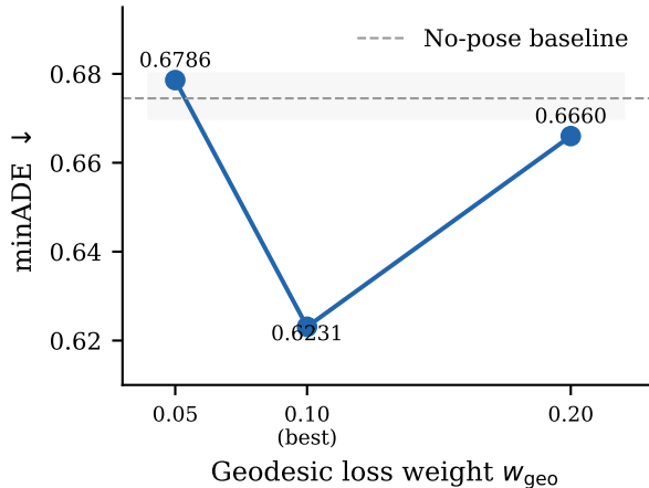
(b) Geodesic loss weight sensitivity
