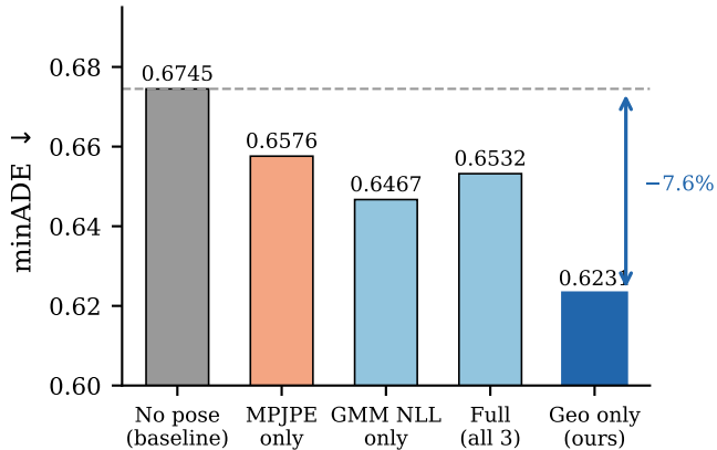
(a) Pose supervision loss ablation
