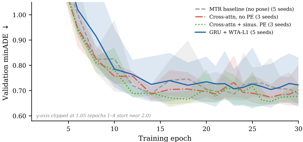
Training dynamics: mean over seeds, band = per-seed range
