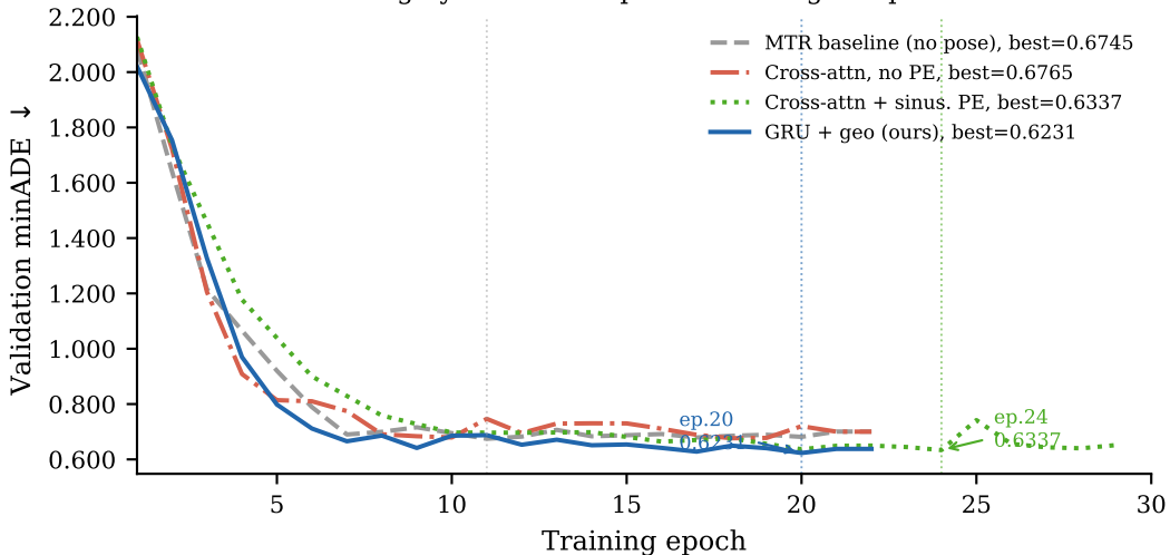
Training dynamics: temporal encoding comparison
