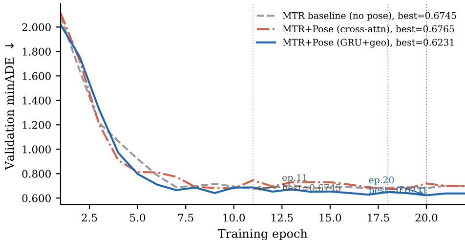
Training dynamics: GRU+geo vs.\ cross-attention vs.\ baseline
