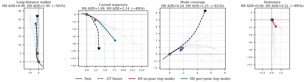
Figure 4: Qualitative comparison at full-Waymo-pretrained scale. Four validation scenes. Past in gray; GT future dashed black with \star endpoint. All 6 predicted modes faded; top-scoring mode highlighted (red: no-pose; blue: geo+pose). Per-scene minADE in titles. Long-distance : no-pose stops at 5m; pose follows the 25m walk. Curved : no-pose underestimates displacement; pose follows the curve. Mode coverage : both top modes underestimate, but pose has a faded mode aligned with GT. Stationary : no-pose wrongly predicts motion; pose correctly stays near origin.
