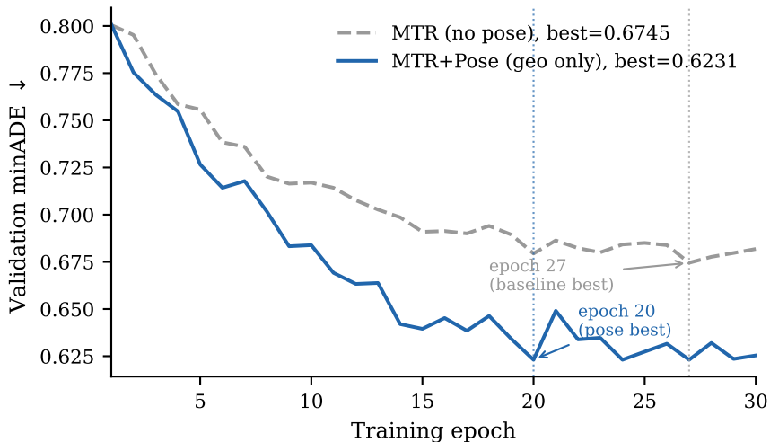
Training dynamics: MTR+Pose vs. baseline
