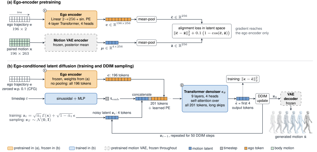
Fig. 1: EgoPed architecture. (a) Ego-encoder pretraining. The ego encoder (1) is trained so that its mean-pooled output \bar{c} matches the mean-pooled posterior mean \bar{z} of the frozen motion VAE for the paired motion. (b) Latent diffusion. The ego encoder is frozen and keeps all 196 per-timestep tokens; for classifier-free guidance the ego input is zeroed for 10% of training samples. At every denoising step, the L = 4 noisy latent tokens z_t , the timestep embedding and the 196 ego tokens are concatenated into one 201-token sequence and processed by a self-attention transformer denoiser (2), whose first four output tokens predict the noise. Sampling runs 50 DDIM steps and decodes z_0 with the frozen VAE decoder; only the denoiser is trained in (b). Section V-E ablates an alternative cross-attention denoiser.
