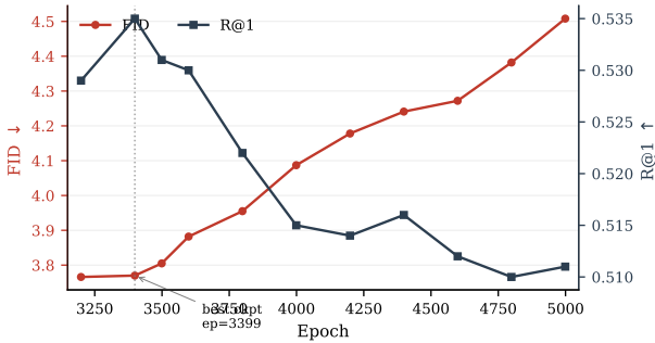
Fig. 5: EgoPed training trajectory: training-time validation FID (left axis, red) and R@1 (right axis, blue) across the late training segment. Epoch 3399 is the best checkpoint (highest R@1, FID within noise of epoch 3199, and best definitive 3-replication FID); both metrics then degrade steadily through epoch 4999. Training loss is flat across this range — sampling quality oscillates independently of training loss.
