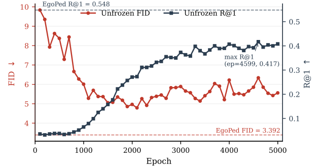
Fig. 4: Unfrozen training trajectory: training-time validation FID (left axis, red) and R@1 (right axis, blue) vs. epoch, over the full 5000-epoch run. FID is best at epoch 2099 and degrades as R@1 rises; after epoch \approx 3299 , R@1 saturates in the 0.37–0.42 band while FID oscillates between 5.1 and 6.3. Dashed reference lines show EgoPed’s best operating point (FID=3.392, R@1=0.548 at epoch 3399, CFG 10). Unfrozen never approaches EgoPed’s performance on either metric.
