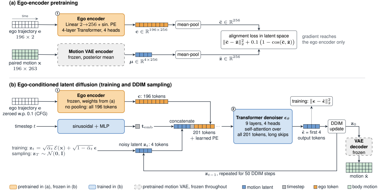
Fig. 1: EgoPed architecture. (a) Ego-encoder pretraining. The ego encoder (1) is trained so that its mean-pooled output \bar{c} matches the mean-pooled posterior mean \bar{z} of the frozen motion VAE for the paired motion. (b) Latent diffusion. The ego encoder is frozen and keeps all 196 per-timestep tokens; for classifier-free guidance the ego input is zeroed for 10% of training samples. At every denoising step, the L = 4 noisy latent tokens z_t , the timestep embedding and the 196 ego tokens are concatenated into one 201-token sequence and processed by a self-attention transformer denoiser (2), whose first four output tokens predict the noise. Sampling runs 50 DDIM steps and decodes z_0 with the frozen VAE decoder; only the denoiser is trained in (b). Section V-E ablates an alternative cross-attention denoiser.
