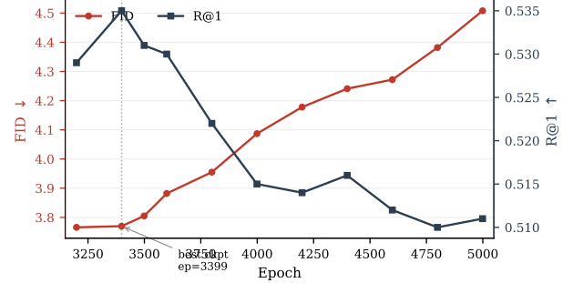
Fig. 4: EgoPed training trajectory: training-time validation FID (left axis, red) and R@1 (right axis, blue) across the late training segment. Epoch 3399 is the best checkpoint (highest R@1, FID within noise of epoch 3199, and best definitive 3-replication FID); both metrics then degrade steadily through epoch 4999. Training loss is flat across this range — sampling quality oscillates independently of training loss.
