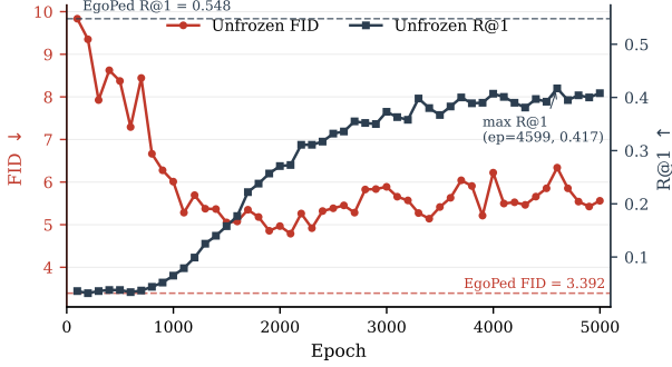
Fig. 3: Unfrozen training trajectory: training-time validation FID (left axis, red) and R@1 (right axis, blue) vs. epoch, over the full 5000-epoch run. FID is best at epoch 2099 and degrades as R@1 rises; after epoch \approx 3299, R@1 saturates in the 0.37–0.42 band while FID oscillates between 5.1 and 6.3. Dashed reference lines show EgoPed’s best operating point (FID=3.392, R@1=0.548 at epoch 3399, CFG 10). Unfrozen never approaches EgoPed’s performance on either metric.
